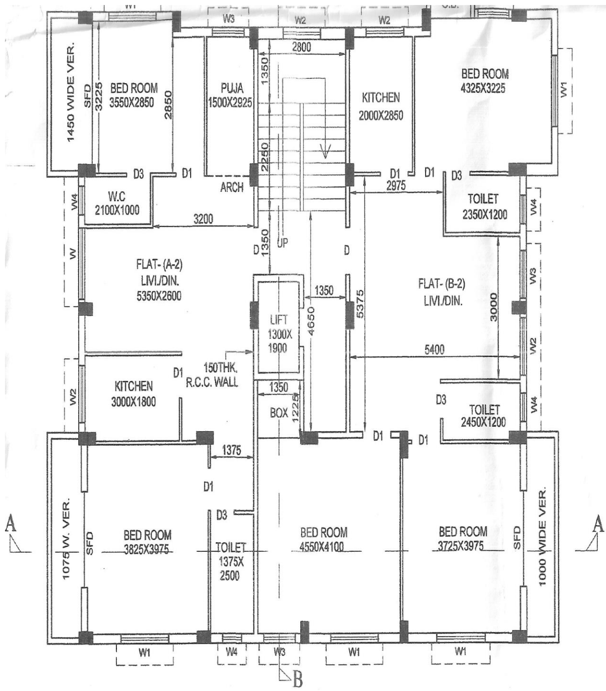
2ND. FLOOR PLAN SCALE - 1:100
